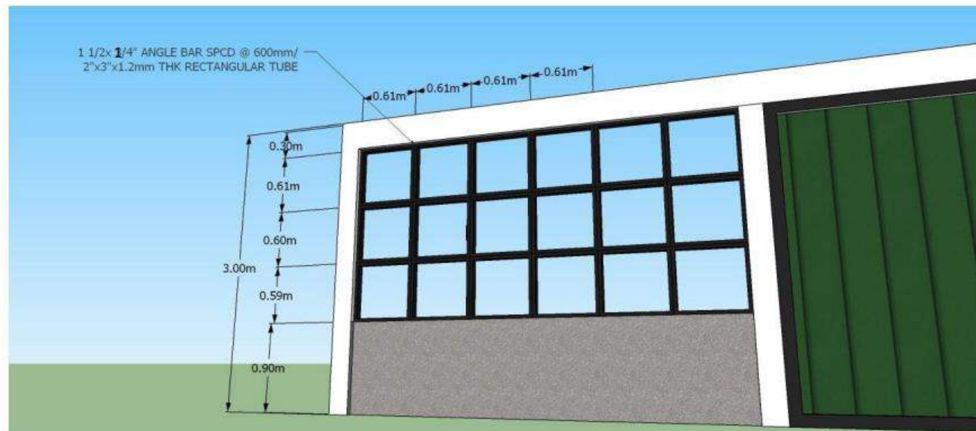
WALL DETAILS
