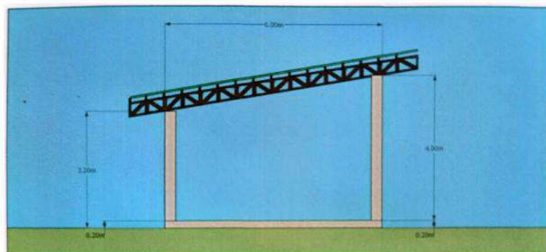
LEFT ELEVATION
