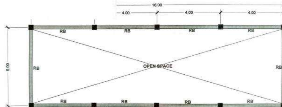
ROOF BEAM PLAN SCALE @ 1:100 METERS
