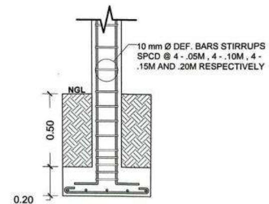
CF DETAIL SCALE @ 1:20METERS
