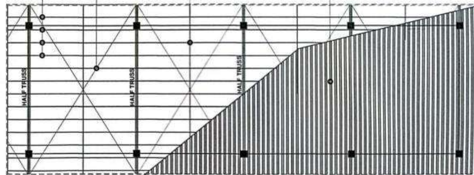
ROOF FRAMING PLAN SCALE @ 1:100 METERS
