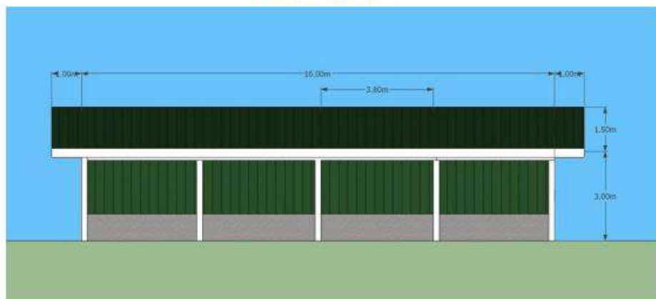
REAR VIEW
