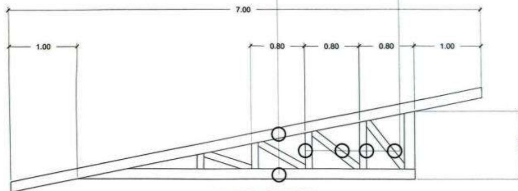
HALF TRUSS DETAIL SCALE @ 1:40METERS
