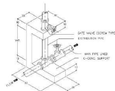
ISOMETRIC DRAWING OF CONCRETE SUPPORT TYPICAL DETAIL OF DISTRIBUTION OUTLET SCALE: 1: 10 MTS.
