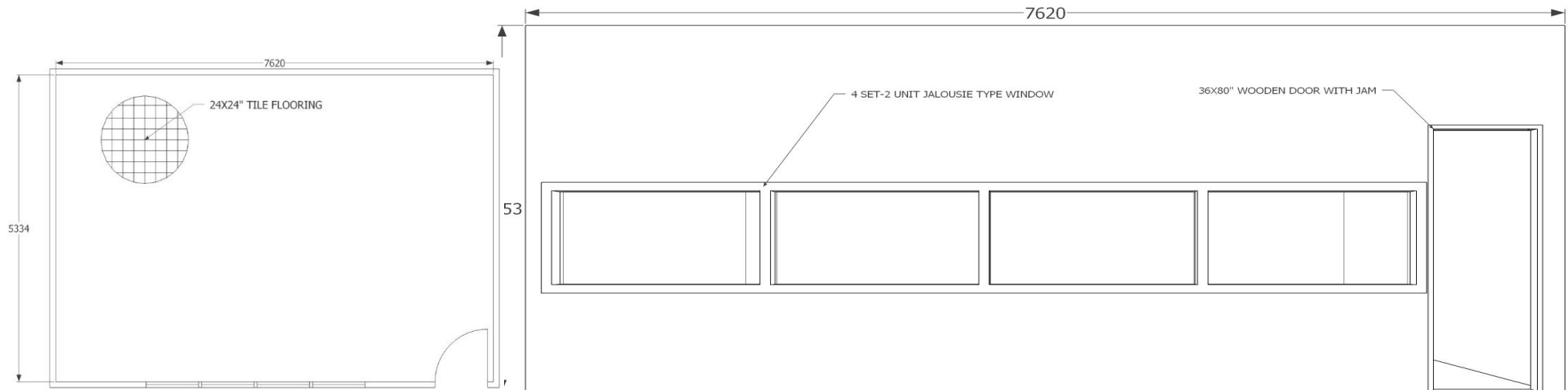
FLOOR PLAN
