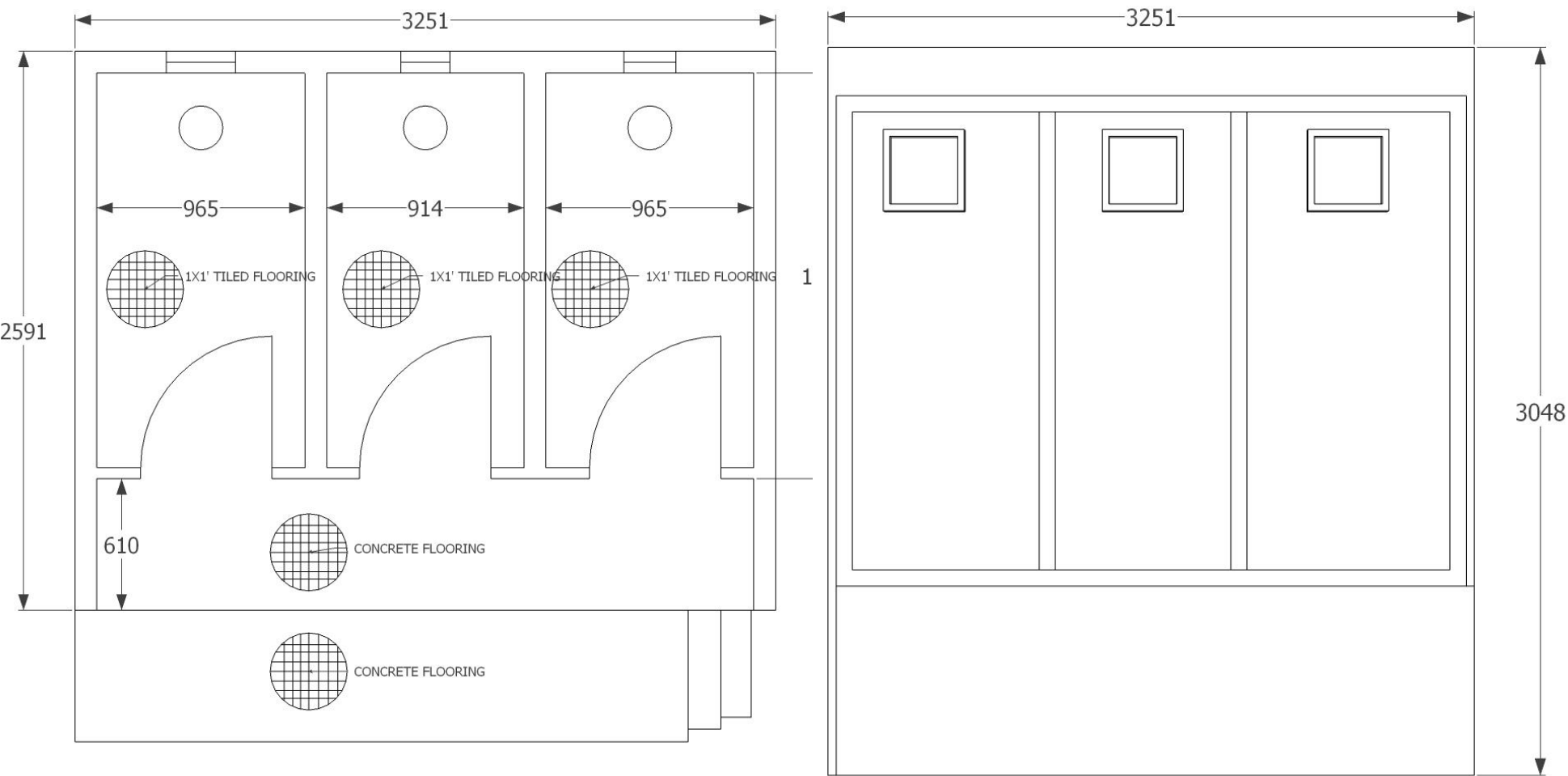
FLOOR PLAN
