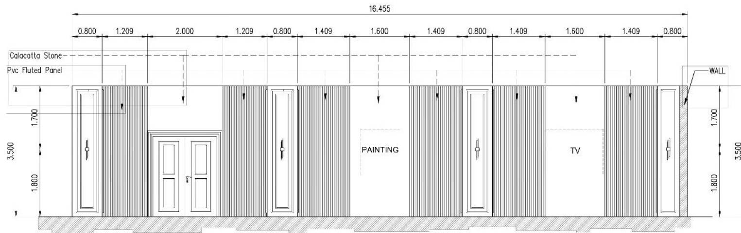
SECTION THRU " C "
