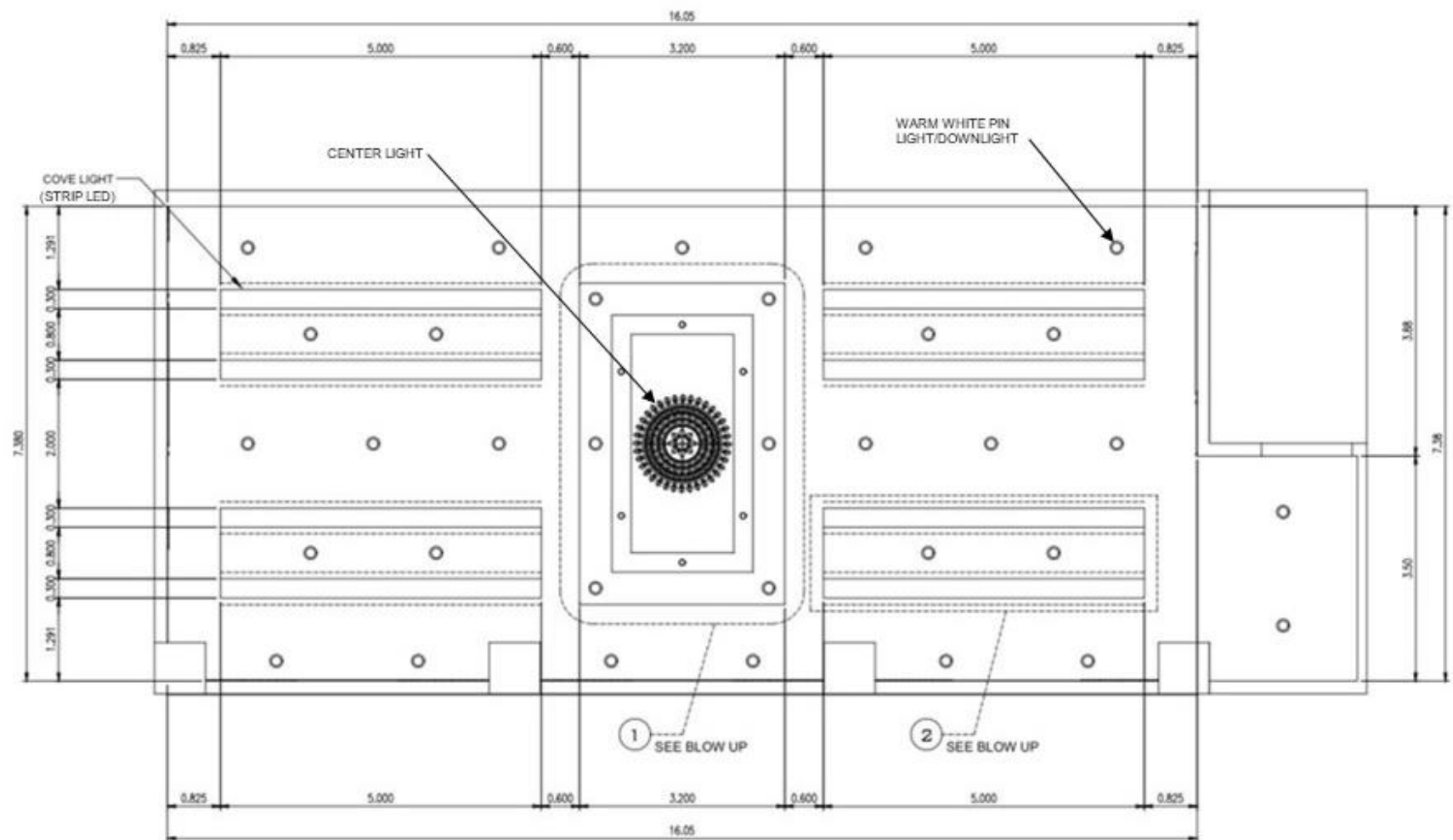
REFLECTED CEILING PLAN Scale: 1:50 METERS
