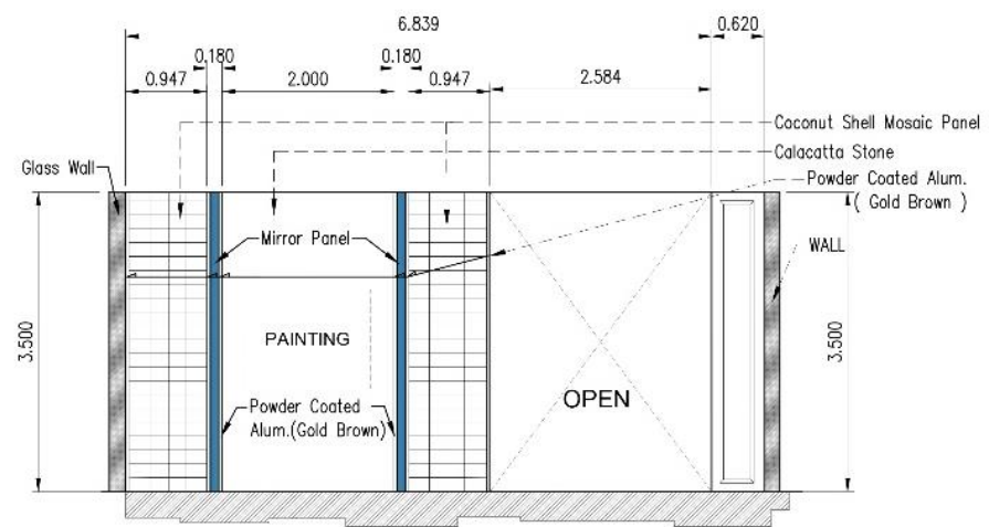
SECTION THRU " B "
