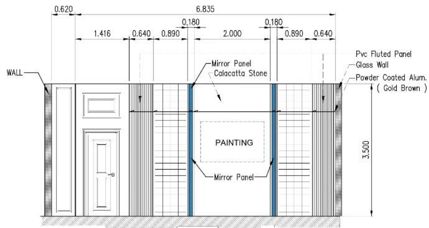
SECTION THRU " A "
